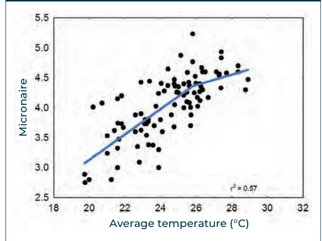
FIGURE 19.1 The response of micronaire to daily average temperature during fibre thickening taken from planting time studies. Varieties used in this study had an average micronaire of 4.05 generated at an average daily temperature of 24.4°C. Adapted from Luo, Bange and Johnston (2014)
