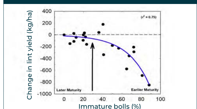
FIGURE 20.3 Effect of early application of harvest aids on lint yield (adapted from Bange et al. 2009). Yield is reduced if defoliation occurs where there are more than 29% immature bolls.
