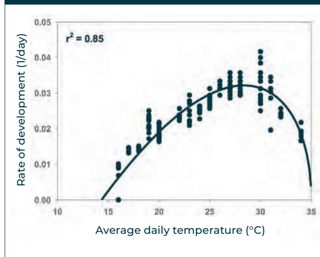
FIGURE 1.1 How quickly cotton develops is impacted by temperature. This graph shows the development rate (comparing the daily fraction of growth up to first square for a range of average temperatures) under controlled environment conditions in a glasshouse.
