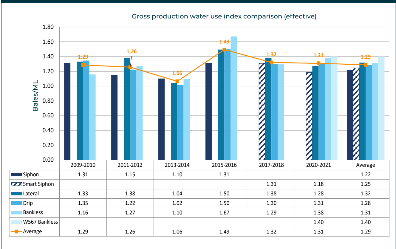
FIGURE 5.6 Keytah system comparison GPWUI summary.
