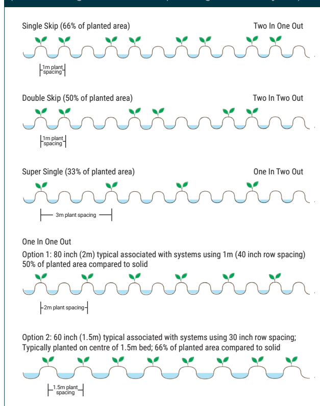
FIGURE 5.3 Alternative row configurations.
