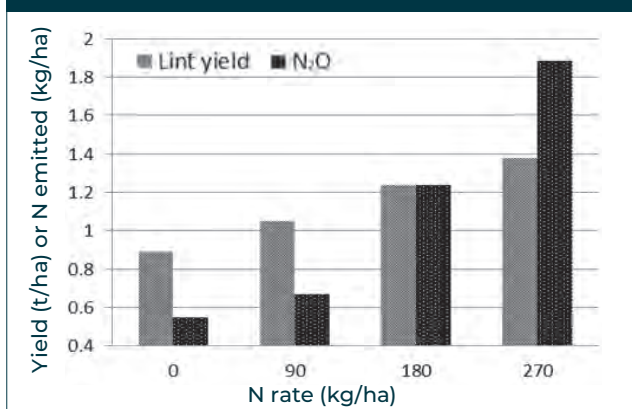
FIGURE 8.2 Cumulative nitrous oxide (N 2 O) emissions and lint yield in response to N application on cotton at Kingsthorpe (Qld) on heavy black clay in 2010-11. (Source: Scheer, et al 2013)
