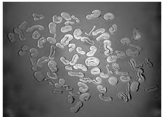
Cross-section of a cotton yarn showing the packing and interaction of individual fibres. Changes in micronaire affect how many fibres make up the cross section of the yarn, impacting its strength and dye uptake. © CSIRO
