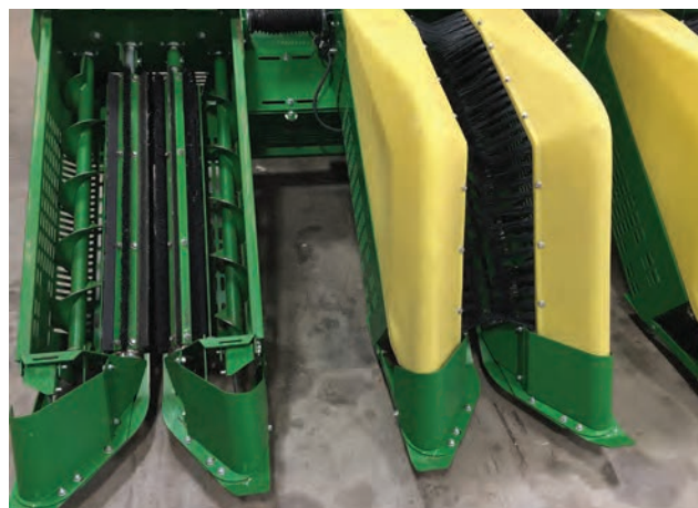
The stripper uses brushes and bats to strip seed cotton from bolls. © René van der Sluijs
