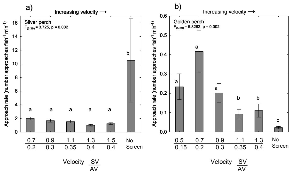
Figure 15. Mean ( \pm SE) rate that a) silver perch and b) golden perch approached the experimental screen across the various slot (SV) or approach (AV) velocities (m/sec) and no screen treatment. Different letters represent significantly different treatments ( p < 0.05 ) determined by pairwise comparisons. Note the different scales on the y axis.
