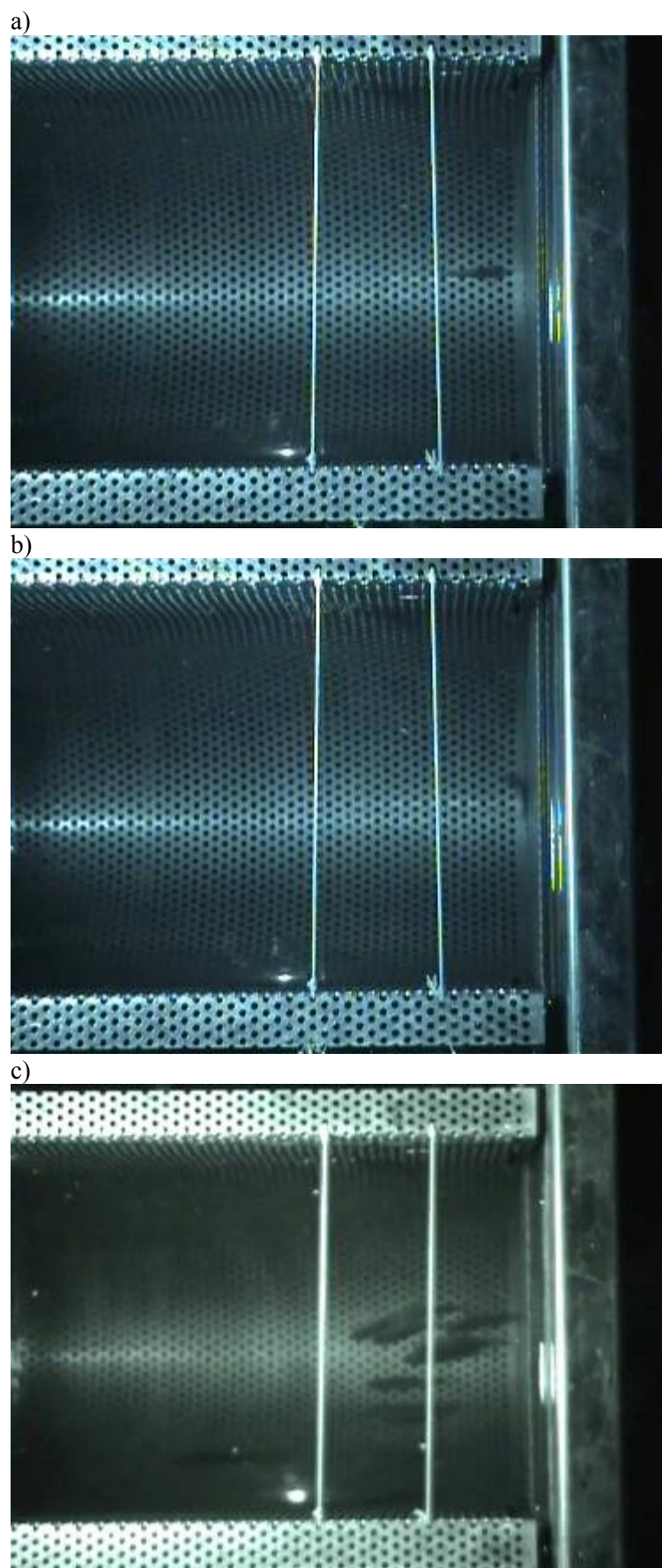
Figure 14. Examples of behaviours commonly observed: a) an approach, b) a contact ( < 3 sec) or impingement (prolonged contact \geq 3 sec), and c) a school of fish displaying positive rheotactic behaviour in front of the screen face.
