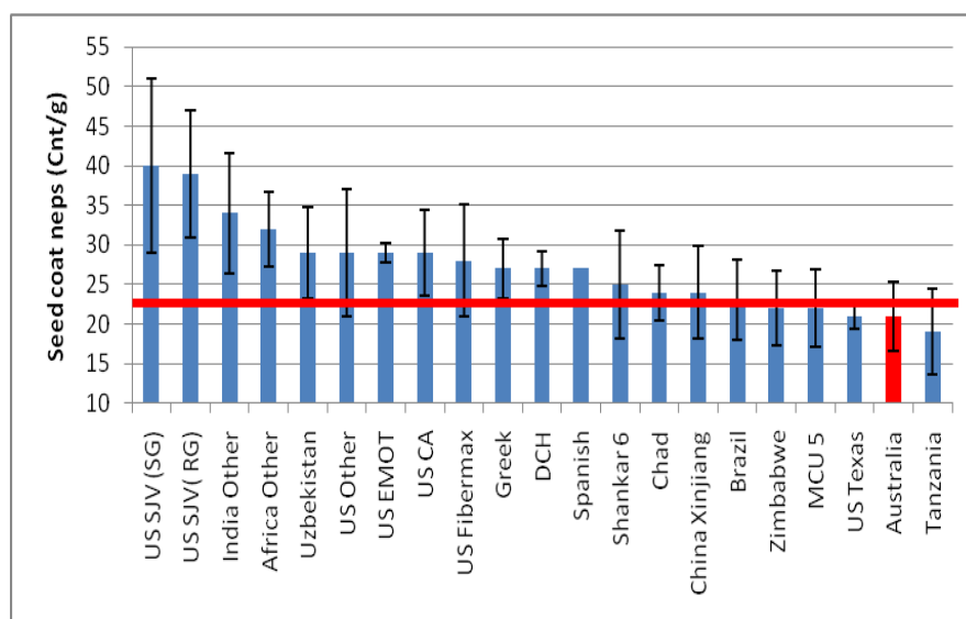
Figure 65 – Average seed coat nep count of bale lay-down samples
