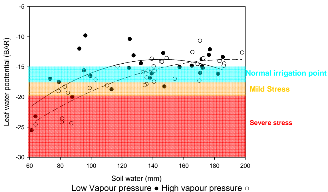
Figure 1. Effect of vapour pressure on leaf water potential, high vapour pressure (○, dashed line) and low vapour pressure (●, solid line). Note that at the same level of soil moisture depending on the atmospheric vapour pressure plants will more or less stressed.
