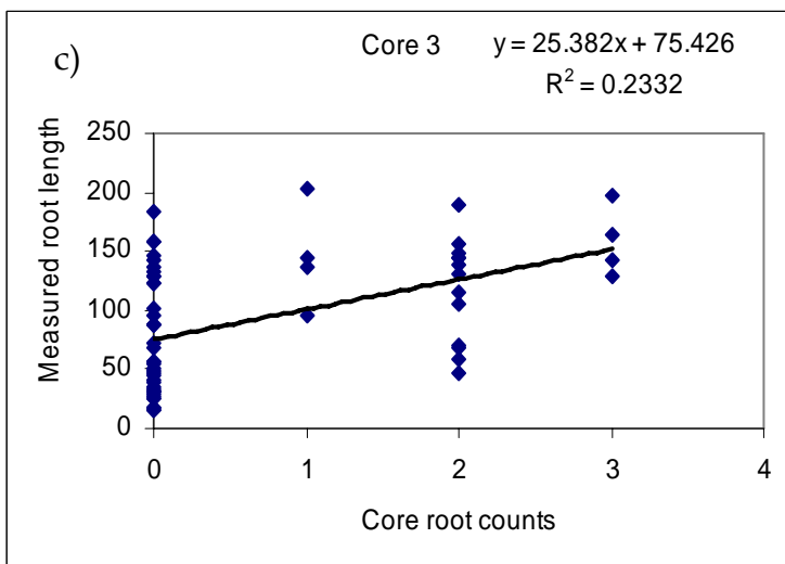
Figure 3. Calibration curves of core breaks compared to measured root length from washed root sample for the three coring times; a) 1st flower, b) cut-out, and c) 60% open bolls in 2006/07 field experiment.
