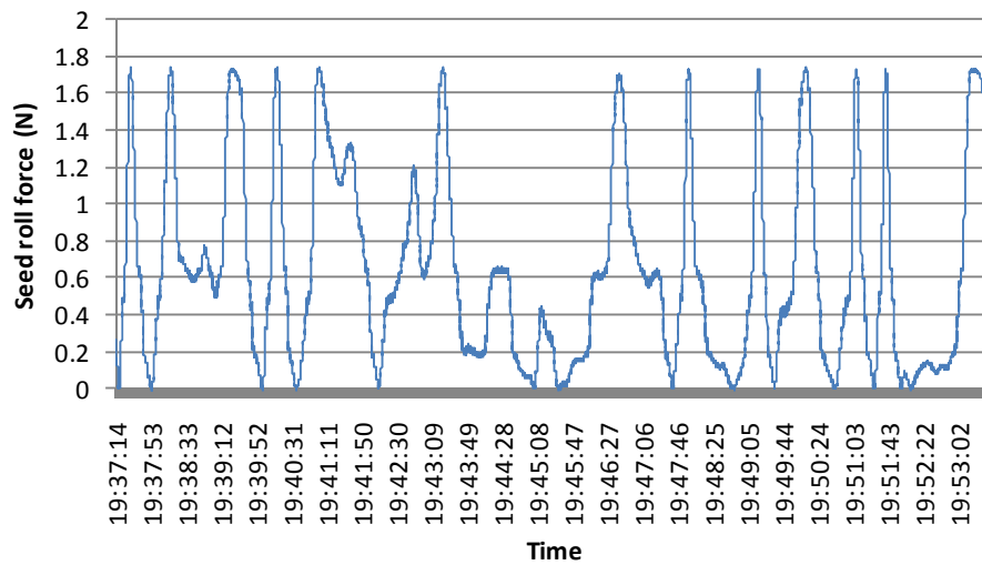
Figure 3-30 Seed roll force capture (20 minute duration).
