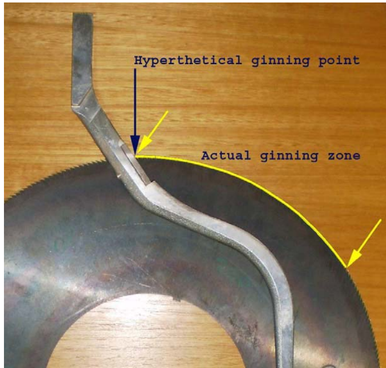
Figure 1-4 Ginning point and ginning zone
