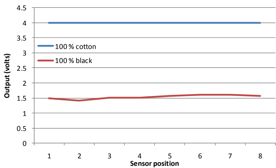
Figure 4-6 DAVS equilibrated calibration
