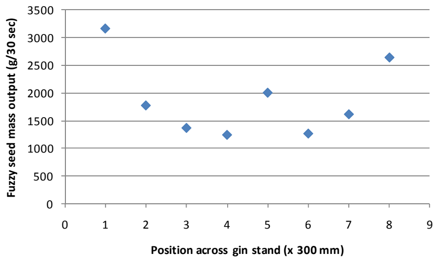
Figure 4-33 Lummus gin stand fuzzy seed output lateral distribution.
