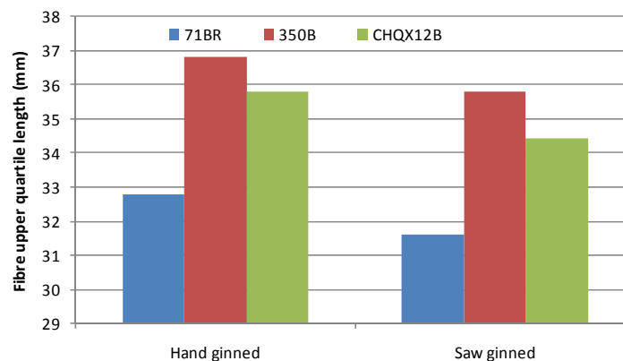
Figure 2-8 Hand ginning vs. saw ginning (UQL).
