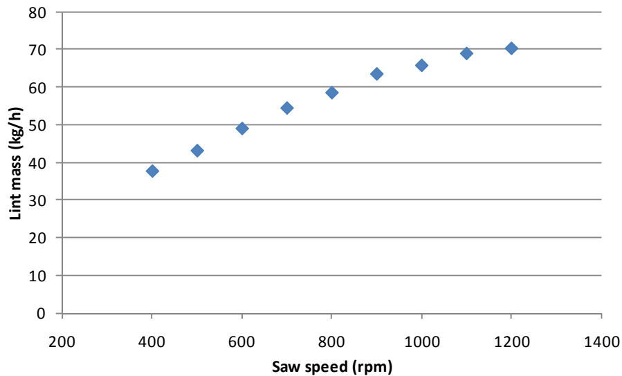
Figure 2-11 Ginning rate & saw shaft rpm.
