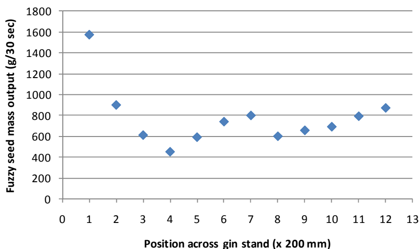
Figure 4-334 Continental Eagle gin stand fuzzy seed output lateral distribution.
