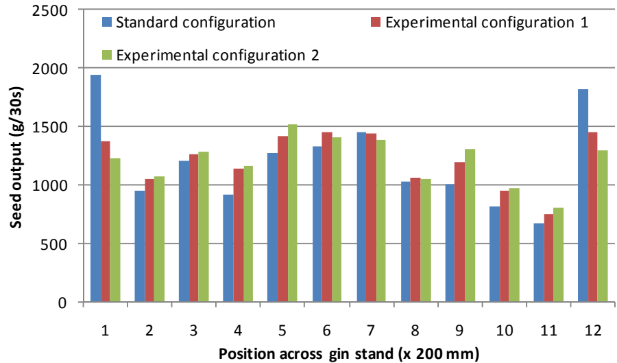
Figure 4-30 Seed cotton flow air manipulation - Double pre cleaner right hand feed.
