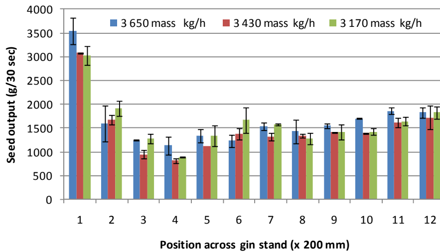
Figure 4-16 Fuzzy seed output distribution from gin stand breast.
