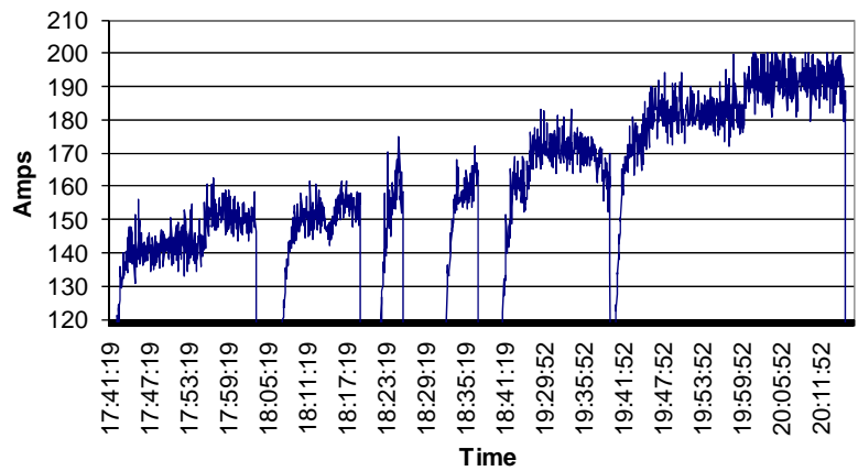
Figure 3-33 Motor current fluctuation at six mass production rates.
