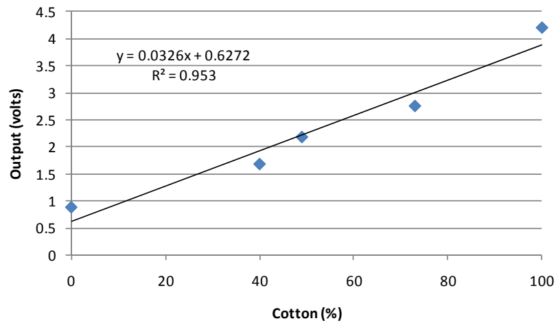
Figure 4-7 DAVS voltage output during five effective surface areas of cotton.
