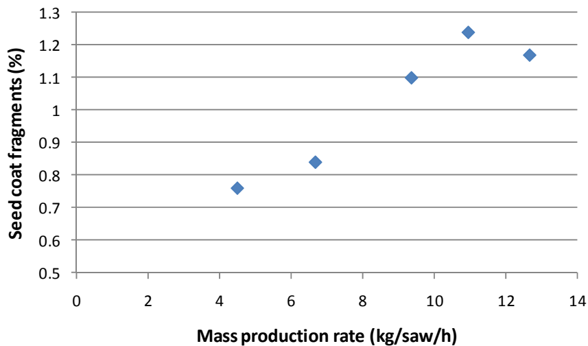
Figure 2-4 Seed coat fragments & ginning rate.
