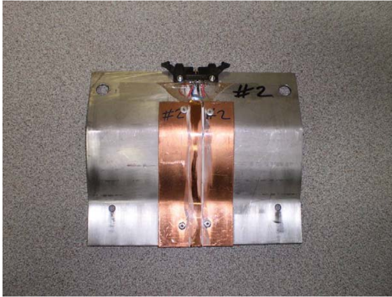
Figure 3-6 Seed roll force sensor mk3.
