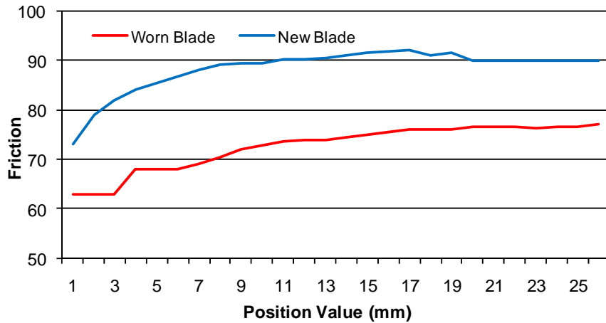
Figure 3-35 Saw blade surface friction – sample 2.
