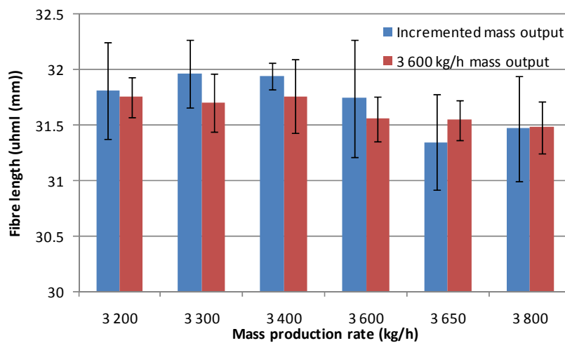
Figure 3-18 T2 uhml results for static and mass production rates
