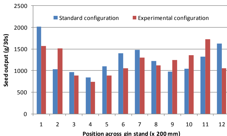
Figure 4-31 Gin stand conveyor distributor modification analyses.
