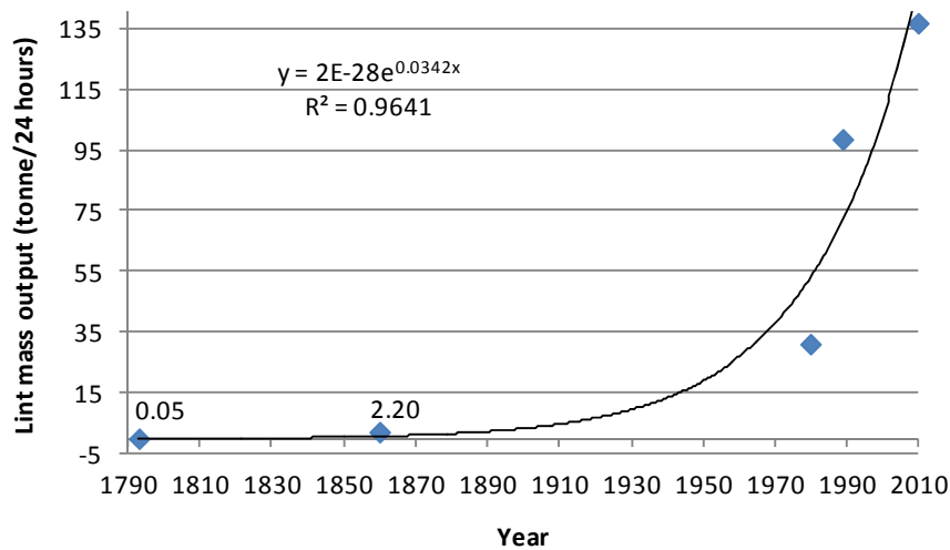
Figure 2-1 Gin stand mass production rate time line.
