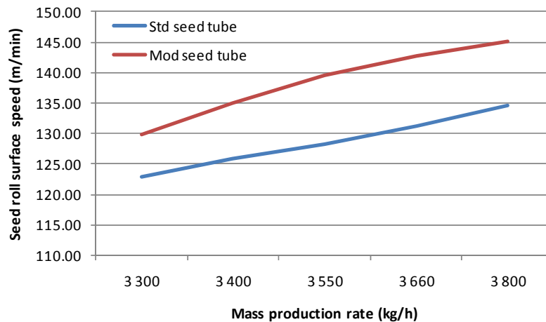
Figure 3-27 Seed roll surface speed.
