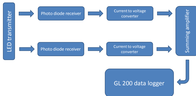
Figure 4-3 DAVS data processing configuration schematic
