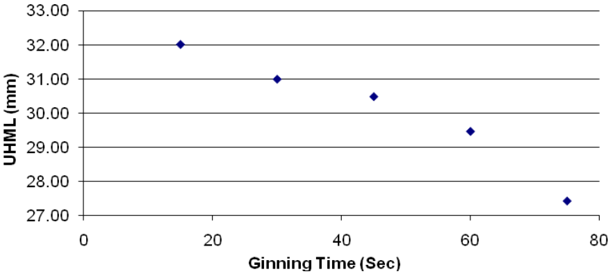
Figure 2-6 Fibre length/ginning time.
