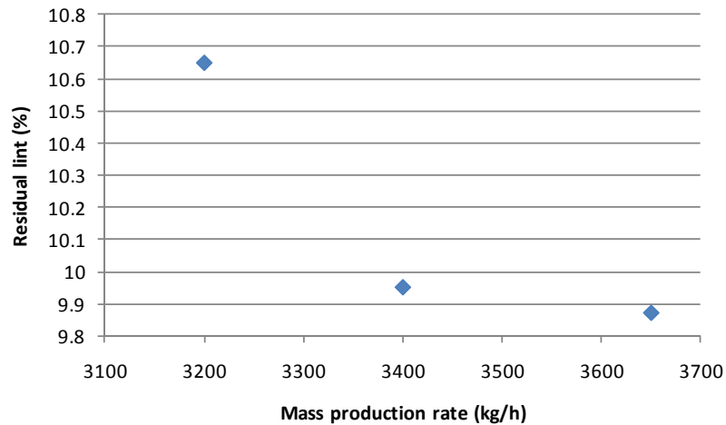
Figure 3-26 Residual lint percentage at three mass production rates.
