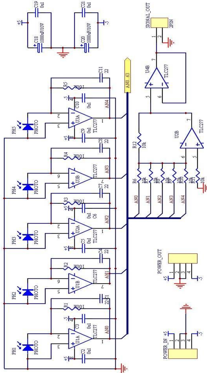
Figure 4-10 DAVS circuit board diagram
