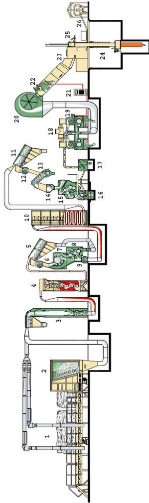
Figure 1-2 Gin layout schematic
