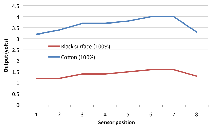
Figure 4-5 DAVS voltage output lab test
