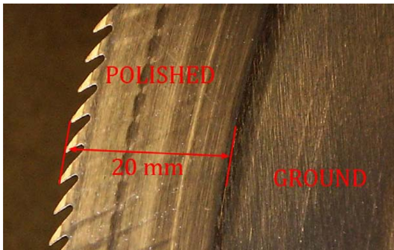
Figure 3-36 Saw blade surface finish.
