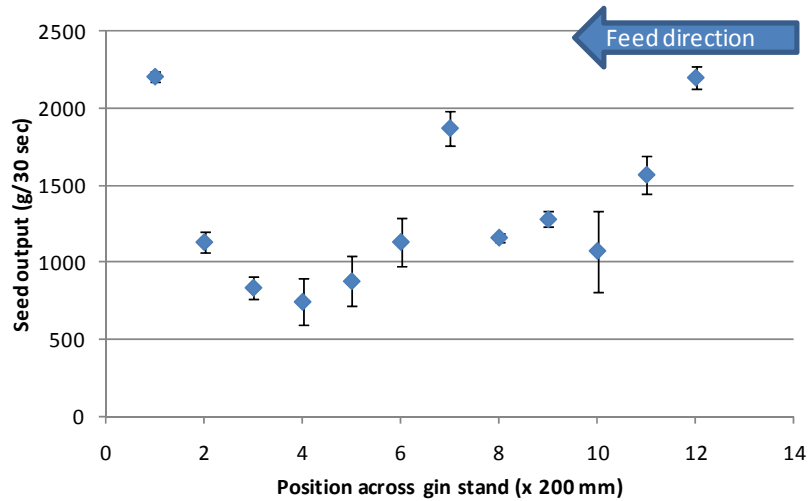
Figure 4-17 Fuzzy seed output distribution (Right hand feed).
