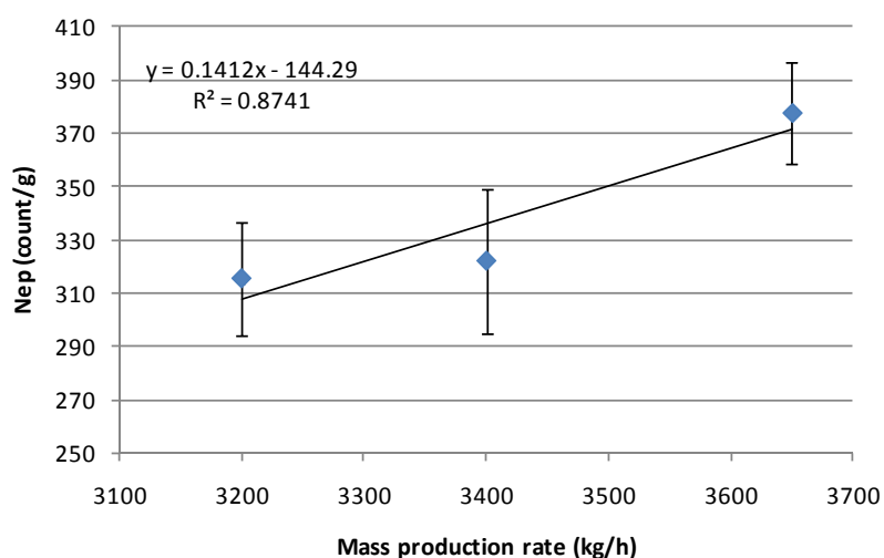
Figure 3-25 Nep formation levels at three mass production rates.
