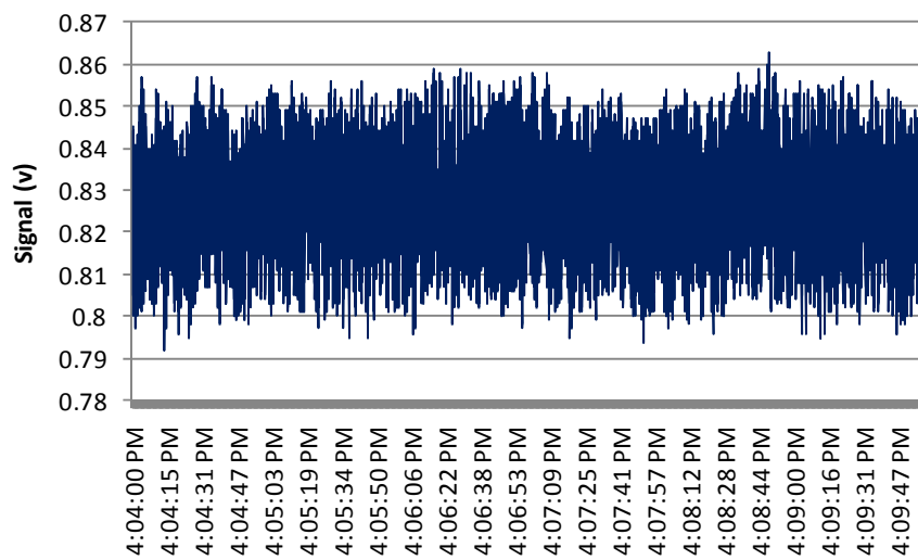
Figure 4-25 DAVS output voltage signal with no material flow.
