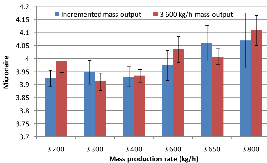
Figure 3-24 T2 micronaire results for static and mass production rates
