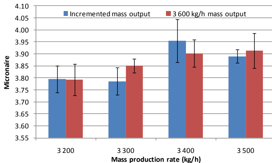
Figure 3-23 T1 micronaire results for static and mass production rates
