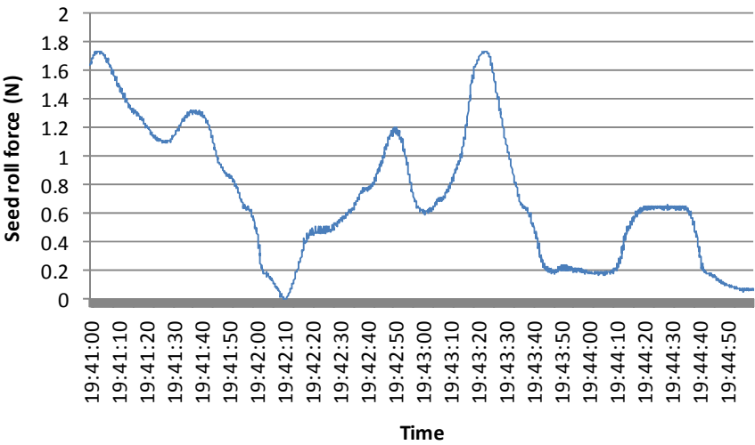
Figure 3-31 Seed roll force capture (4 minute duration).
