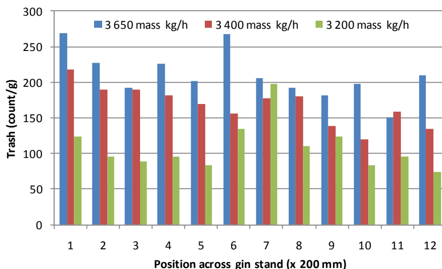
Figure 4-19 Trash count levels across gin stand.
