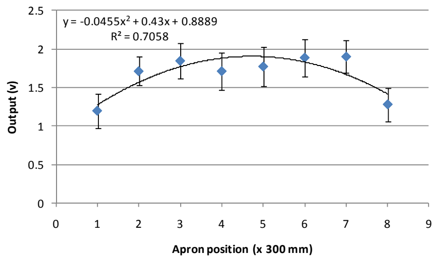
Figure 4-22 DAVS gin stand feed analyses - 2 x pre cleaner, seed cotton feed from the right hand side.
