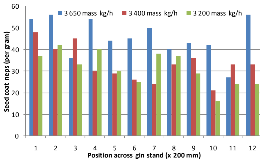
Figure 4-18 Seed coat nep distribution across gin stand.
