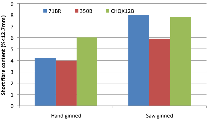
Figure 2-7 Hand ginning vs. saw ginning (SFC).
