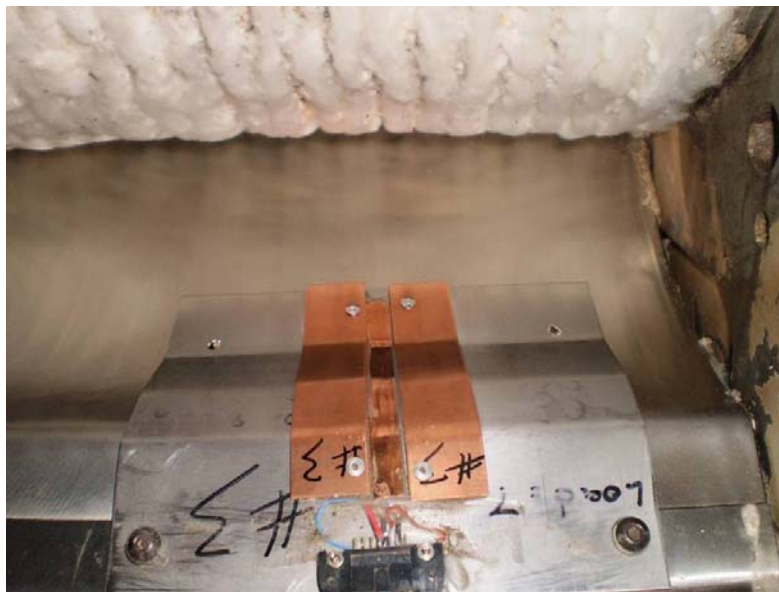
Figure 3-5 Seed roll force sensor positioned within roll box.
