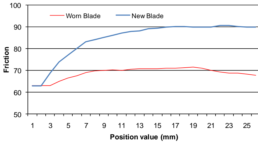
Figure 3-34 Saw blade surface friction – sample 1.
