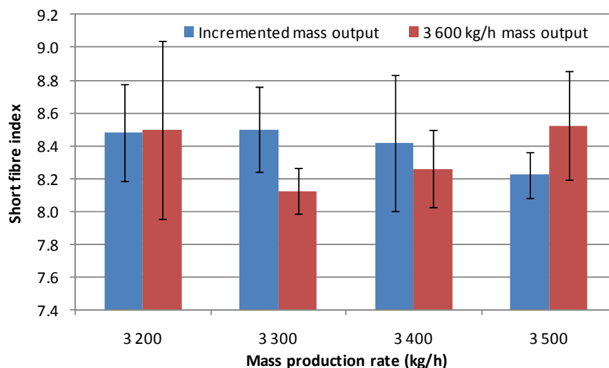
Figure 3-21 T1 short fibre content results for static and mass production rates
