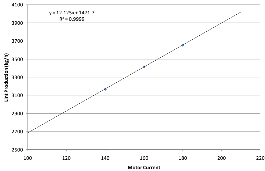
Figure 3-1 Motor current and lint production conversion chart.
