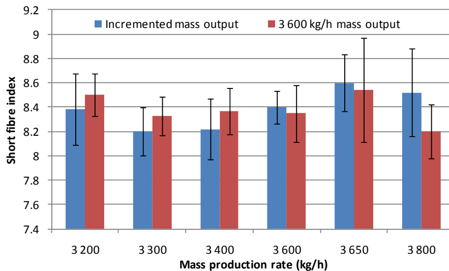
Figure 3-22 T2 short fibre content results for static and mass production rates
