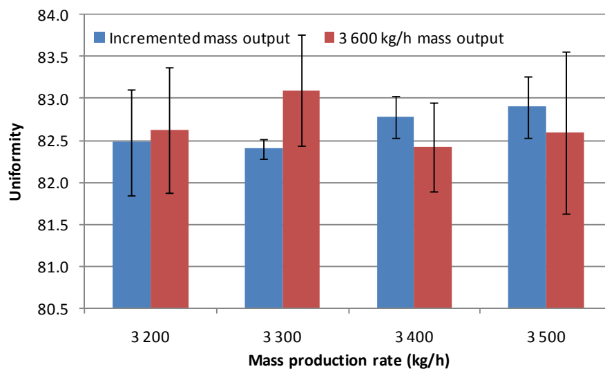
Figure 3-19 T1 uniformity results for static and mass production rates
