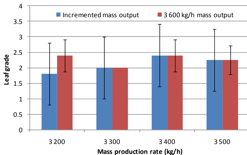
Figure 3-15 T1 Leaf grade results for static and mass production rates
