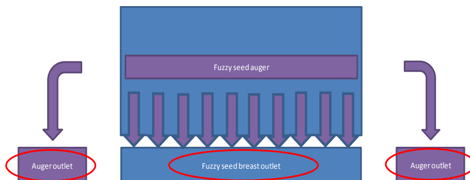
Figure 3-9 Fuzzy seed expulsion zones schematic
