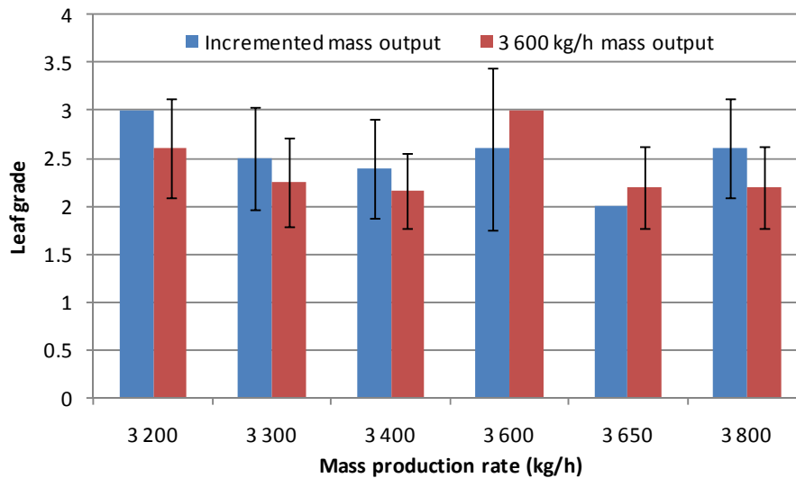
Figure 3-16 T2 Leaf grade results for static and mass production rates
