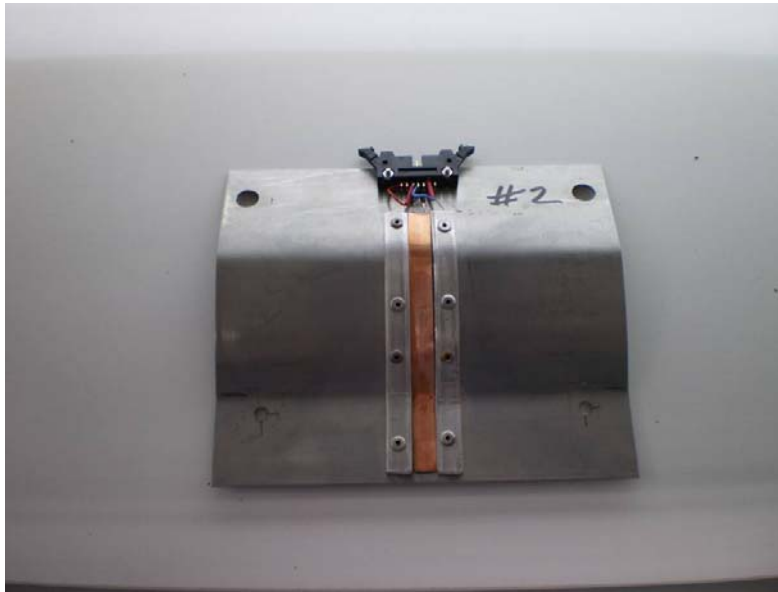
Figure 3-7 Seed roll force sensor mk2.
