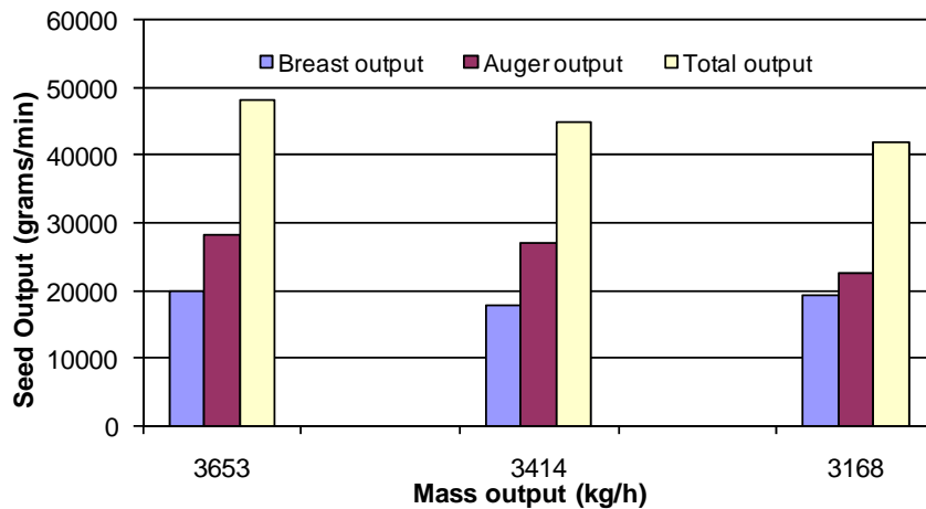
Figure 4-15 Mass fuzzy seed discharge from breast and auger.
