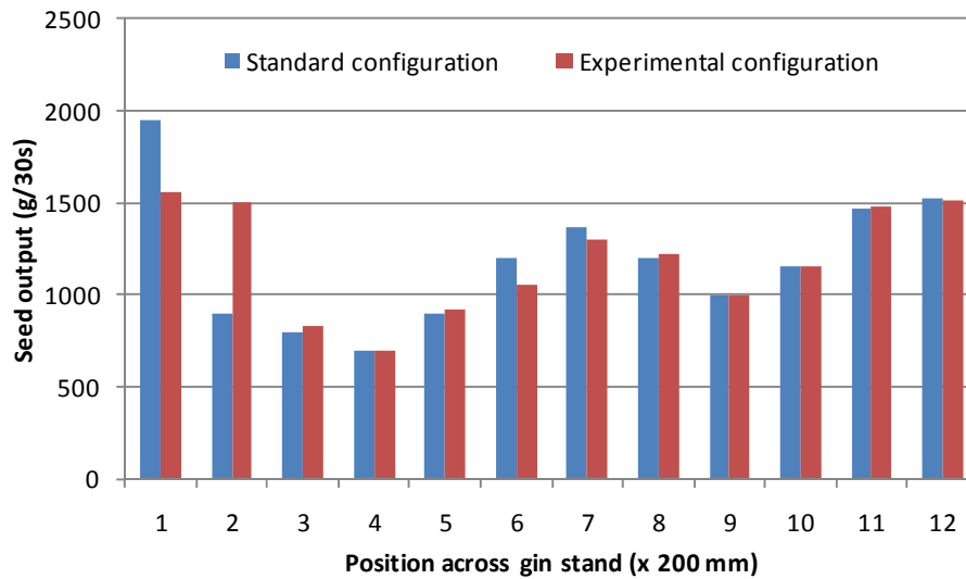
Figure 4-29 Gin stand deflector input distribution.
