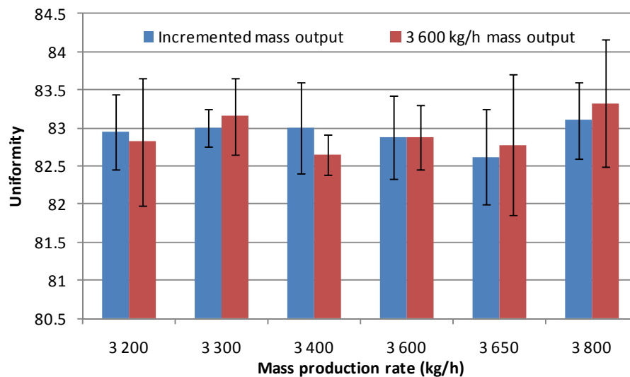
Figure 3-20 T2 uniformity results for static and mass production rates
