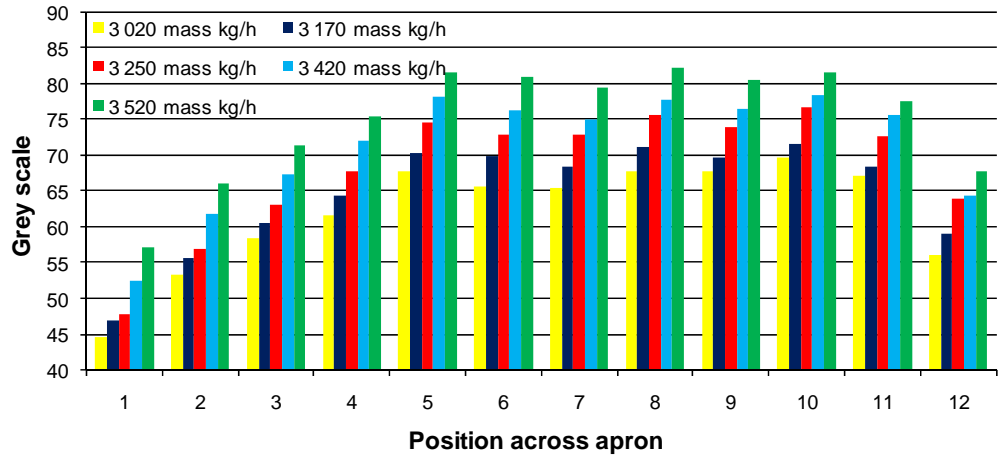
Figure 4-21 Gin stand feeder apron grey scale values.
