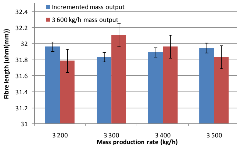
Figure 3-17 T1 uhml results for static and mass production rates
