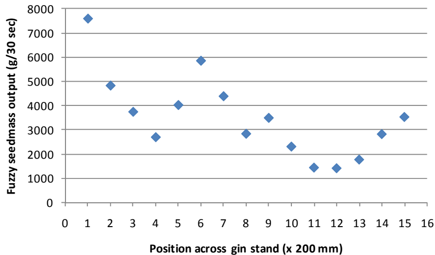
Figure 4-32 Consolidated gin stand fuzzy seed output lateral distribution.
