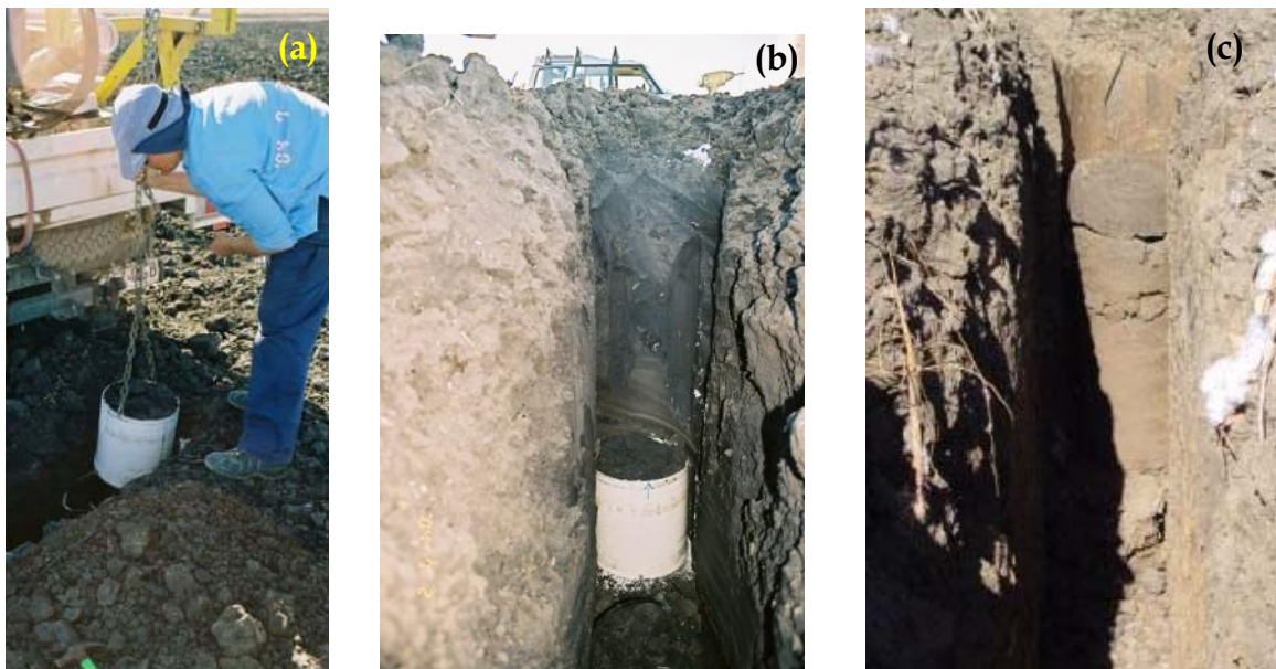
Fig. 4 (a) Lowering the lysimeter back down the hole. (b) The lysimeter in place with plumbed drainage line extending back to the edge of the field (towards the camera). (c), the intact soil cores placed in original order on top of the lysimeter, before the hole and access trench is in
