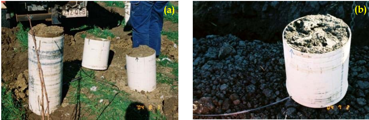
Fig. 3 (a) The three parts of the extracted soil cores. The longer core contains the 0 – 75 cm layer, the two smaller cores contain the 75-105 (right) and the 105-150 cm (center) layer; that becomes the lysimeter. (b) The lysimeter, after plumbing the ceramic candles, silica flour and sealing the base, ready to be lowered back down the hole
