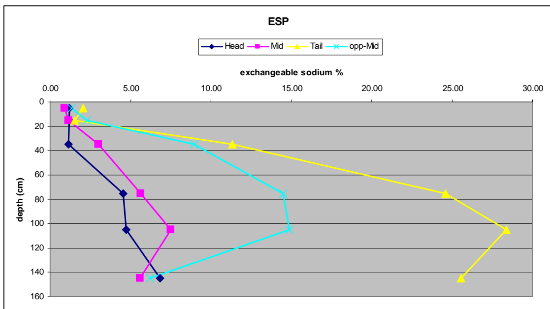
Fig. 4 Exchangeable sodium % (ESP) ie Sodium as a % of the cation exchange capacity (CEC) to 150 cm depth at each of the four lysimeter locations (head, mid, tail and mid-opposite) at the Maules Creek site.
