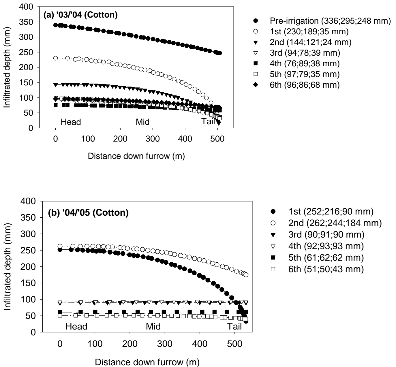
Figure 36 Infiltration uniformity simulated from SIRMOD down the furrow (530 m) on the St George (S) site for 7 and 6 irrigation events in the (a) 2003-4 and (b) 2004-5 cotton seasons. The modelled amounts of water infiltrated at each head, mid and tail locations are also shown in the legend. Note; no data available for pre-irrigation during 2004-05 season.
