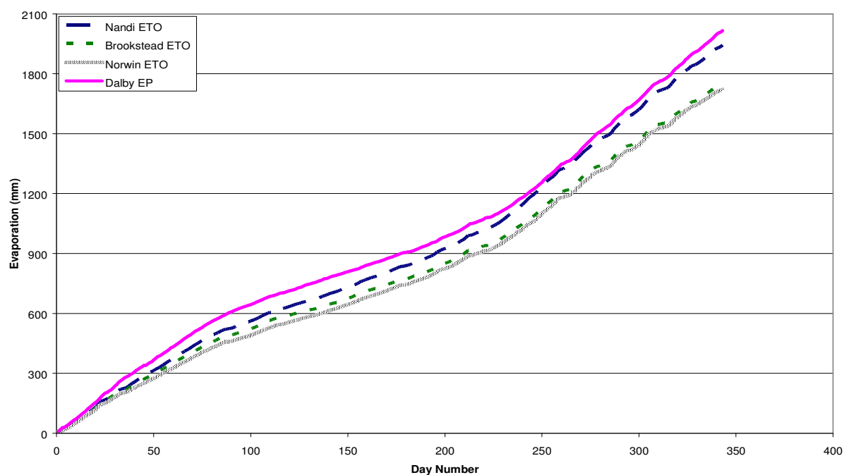
FIGURE 12 – CUMULATIVE AWS AND CLASS ‘A’ PAN EVAPORATION (DALBY)
