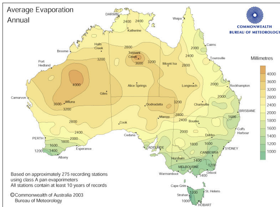
FIGURE 7 - AVERAGE ANNUAL PAN EVAPORATION FOR AUSTRALIA
