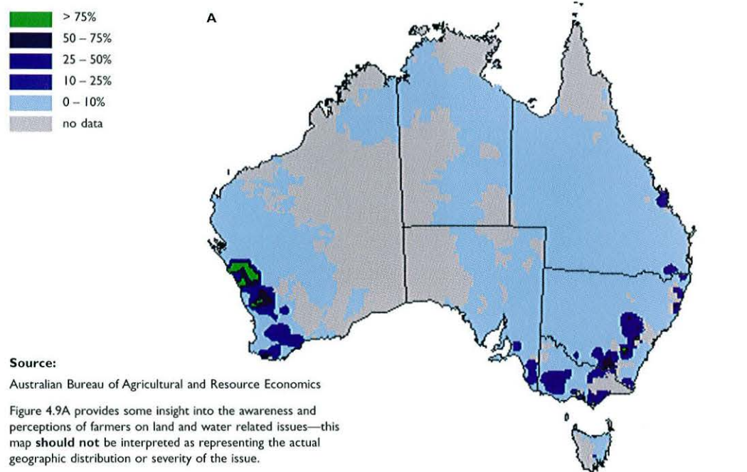
Figure 4.9 Proportion of farms with soil acidity problems, 1998/99 showing (A) farmer perceptions and (B) acidity yield loss (at least 5%) areas.
