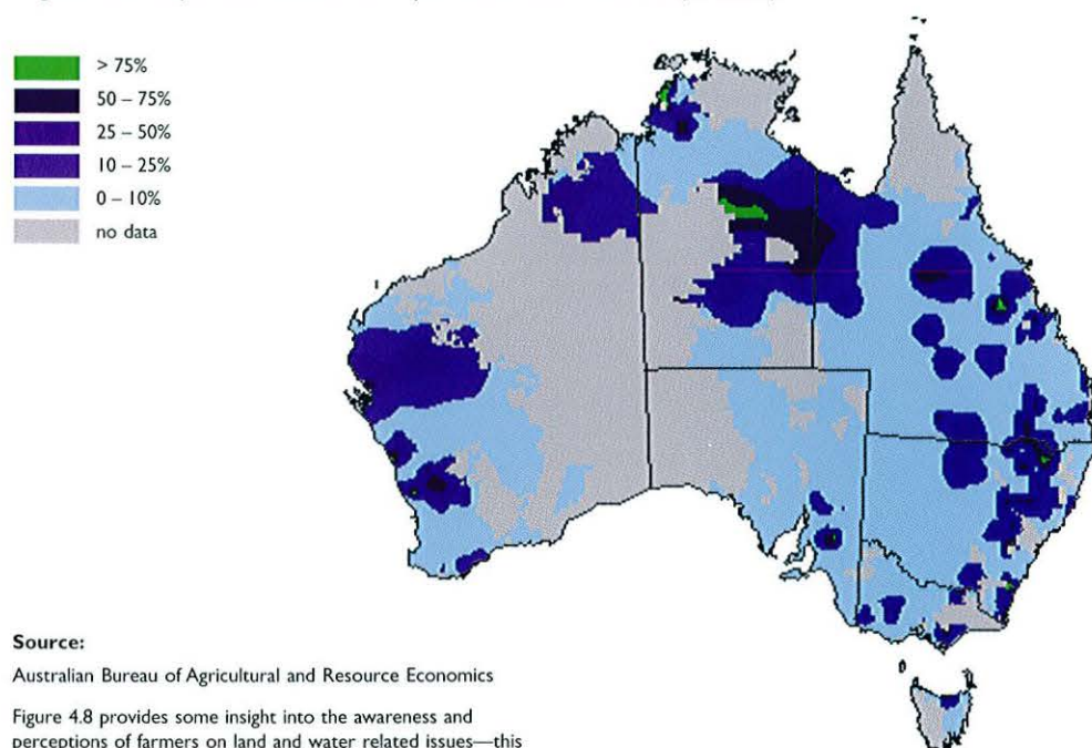
Figure 4.8 Proportion of farms with perceived water erosion (1998/99).
