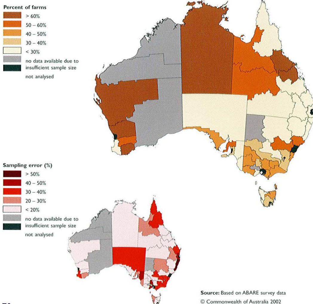
Figure 3.4 Membership of Landcare in 1998/99.
