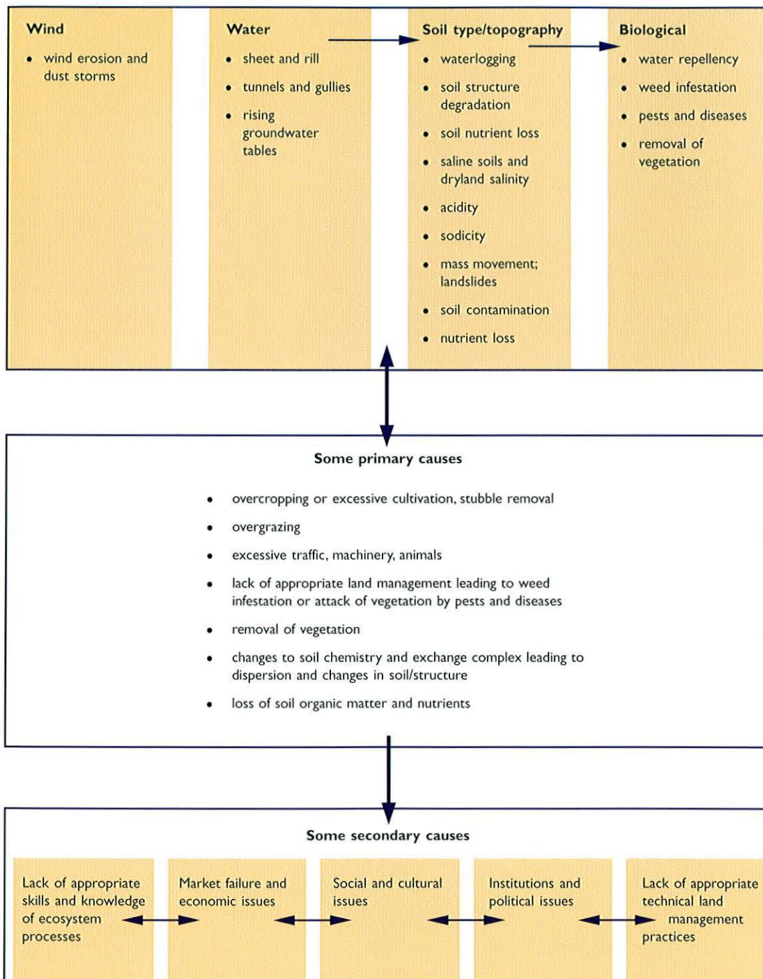
Figure 4.3 Some types and causes of land degradation.
