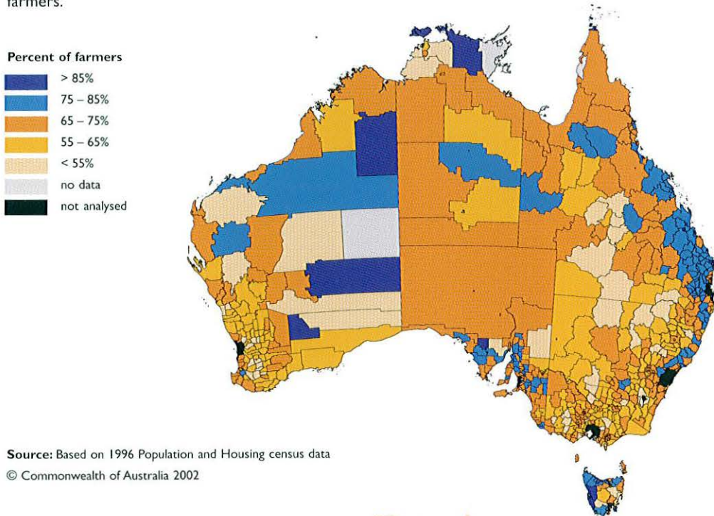
Figure 3.3 Farmers aged 14–16 years when they completed their formal schooling as a percentage of all farmers.
