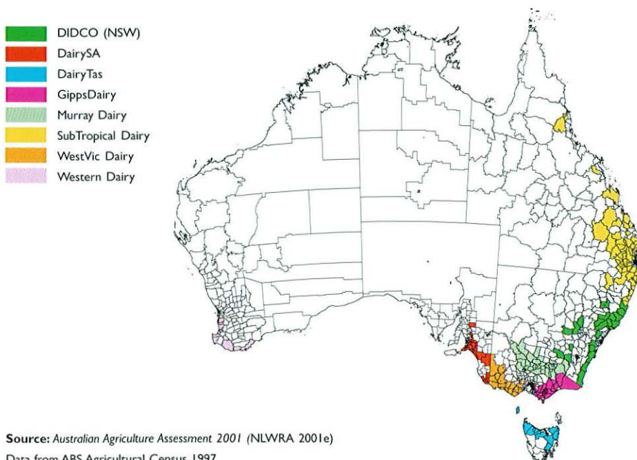
Figure 7.7 Major dairying regions in Australia in 1996/97.
