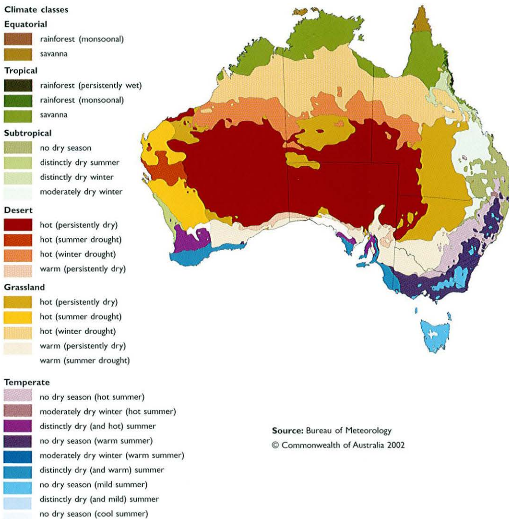
Figure 1.1 Australia's climate zones.
