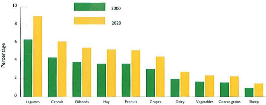
Figure 4.5 Proportion of specific land uses currently affected by dryland salinity.
