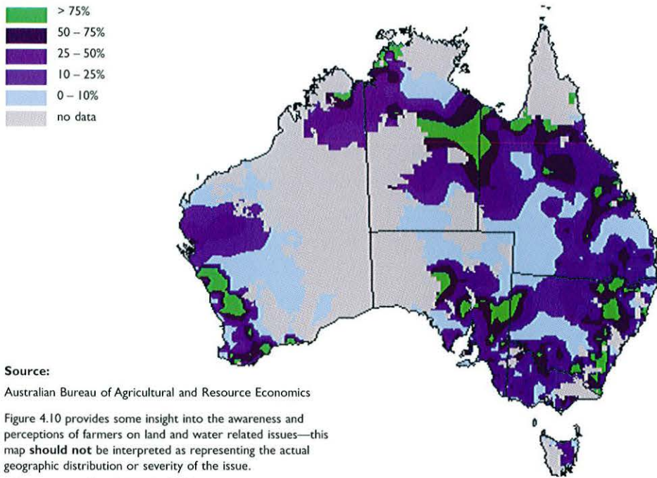
Figure 4.10 Proportion of farms indicating at least one significant degradation problem.
