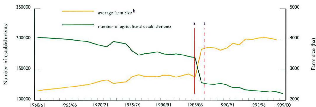
Figure 1.19 Change in farm number and area (1960–2000).
