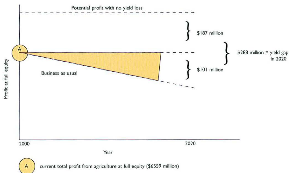
Figure 4.6 Interpretation of the current and future yield gap values for dryland salinity.
