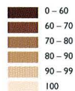
Figure A5 Relative yield from salinity in 2020 (%).
