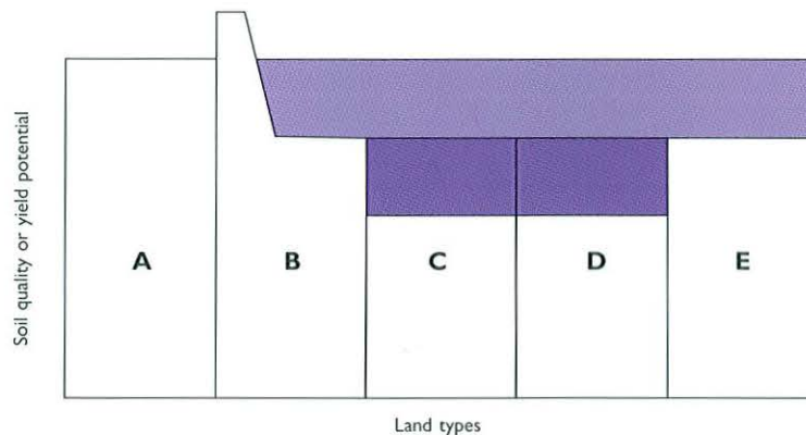
Figure 4.1 The concept of land degradation.
