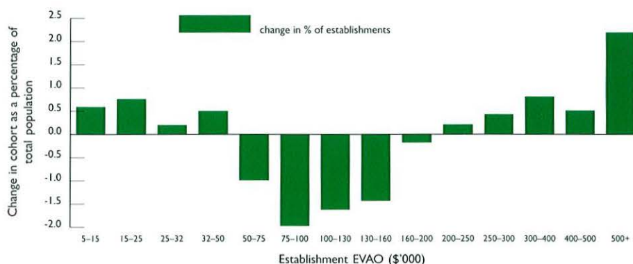
Figure 3.5 Change in number of farm establishments by estimated value of agricultural operations (EVAO) grouping as a percentage of all farm establishments 1986 to 1996 (using constant 1996 dollars).
