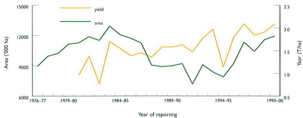
Figure 1.10 Wheat yield and area.
