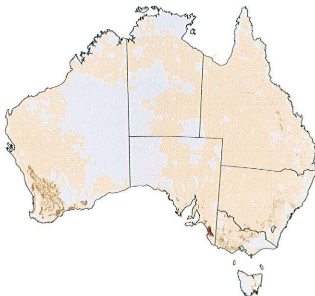
Figure A5 Relative yield from salinity in 2020 (%).
