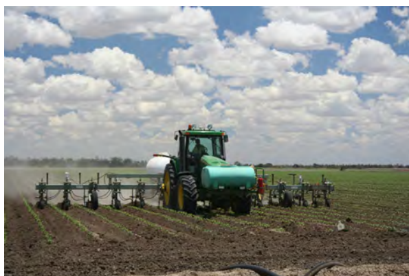
Inter-row cultivation rig set up for one-pass cultivation and cold-flow nitrogen application.
