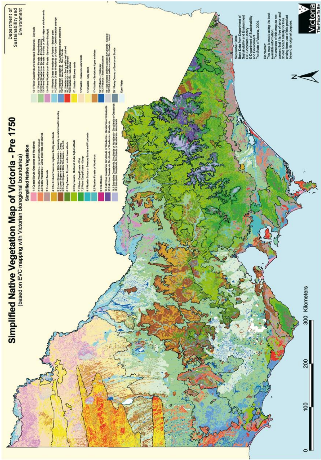
Figure 2.1: The pre-European landscape
