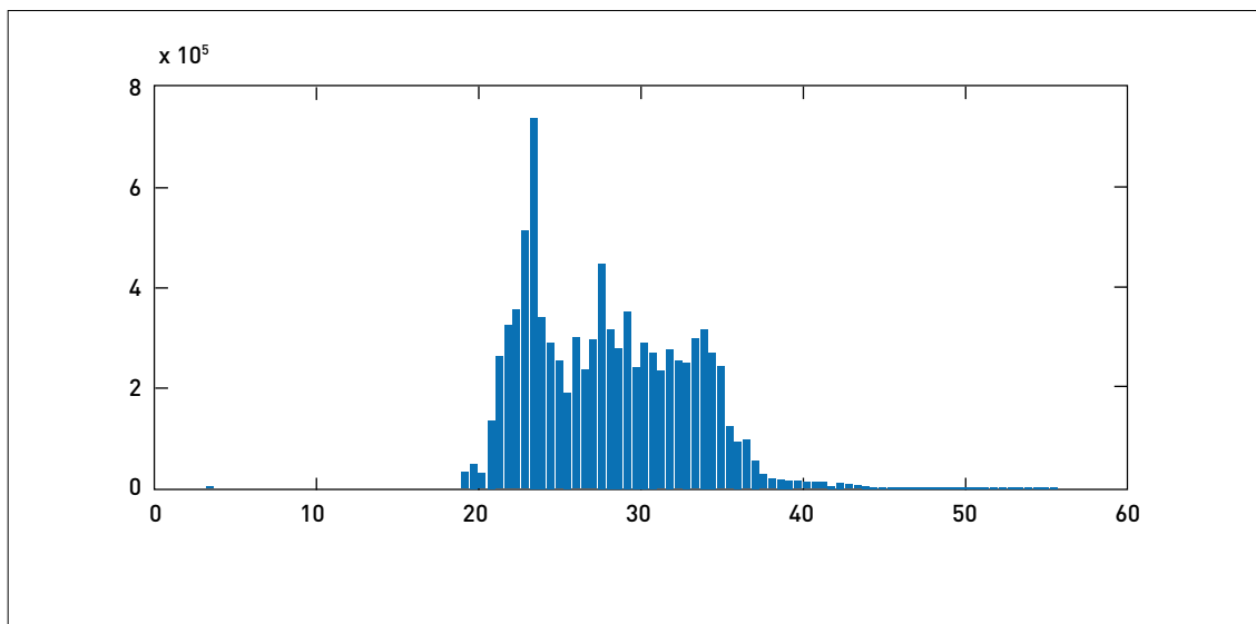
Figure 2.13: Distribution of mean annual carbon – pre-European landscape (kg/m 2 /yr)
