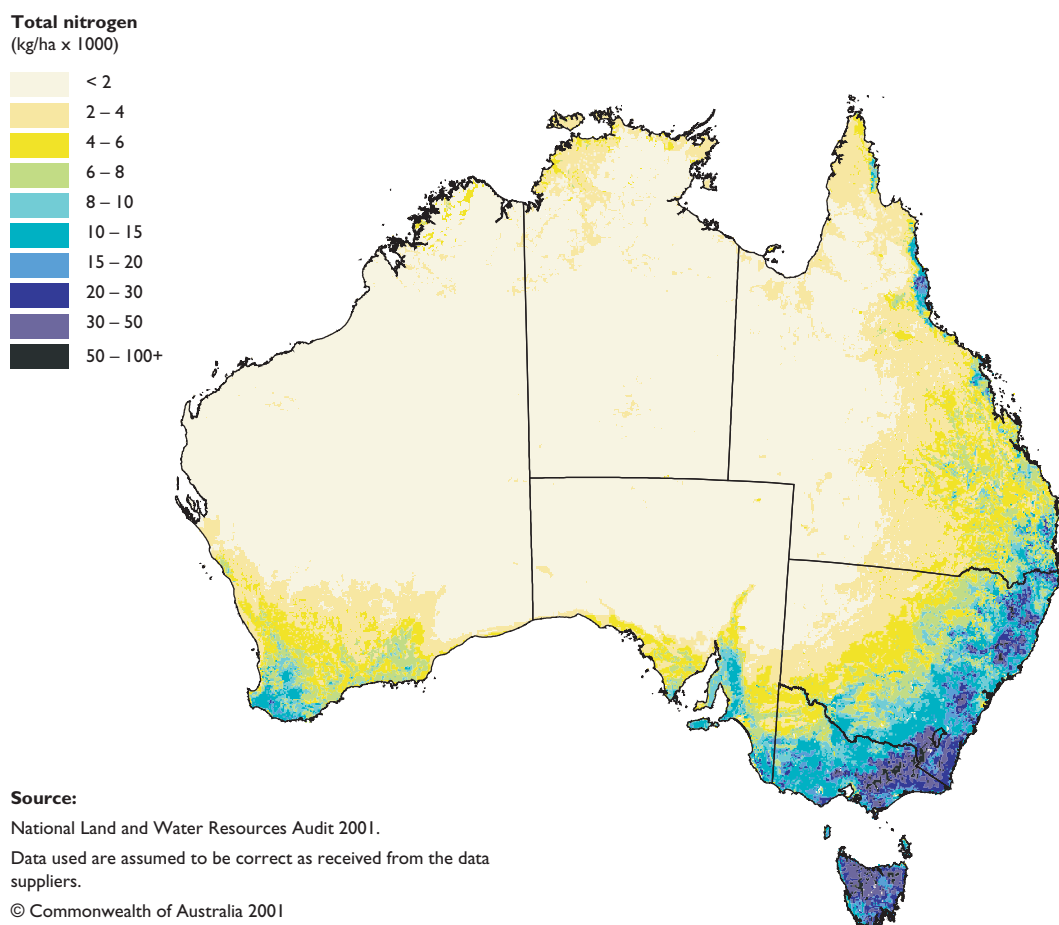
Figure 2.19 Steady-state store of total plant available nitrogen, consisting of organic nitrogen in litter and soil plus the mineral plant-available nitrogen (including both ammonium and nitrate) under current agricultural practices.
