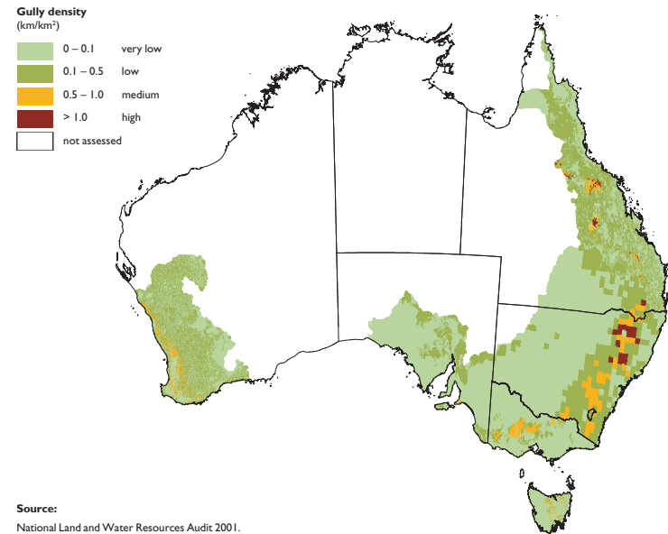
Figure 5.10 Gully density.
