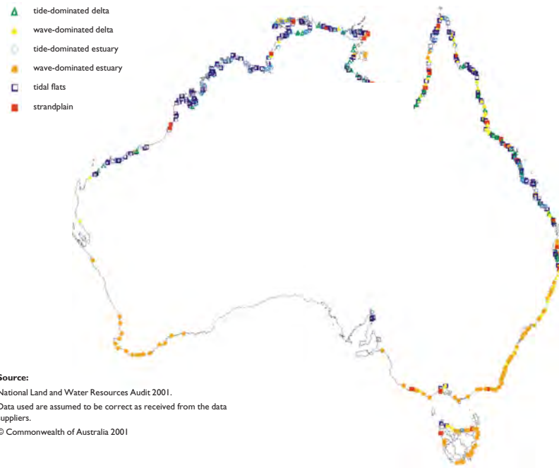
Figure 6.2 Australian estuary types.
