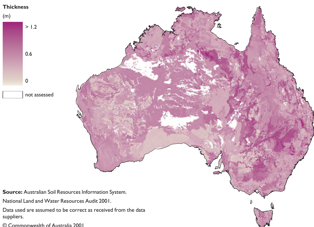
Figure A6 Distribution of depth of first subsoil (m) across Australia.
