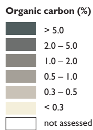
Figure A15 Distribution of organic carbon (%) in the subsoil within the river basins containing intensive agriculture.
