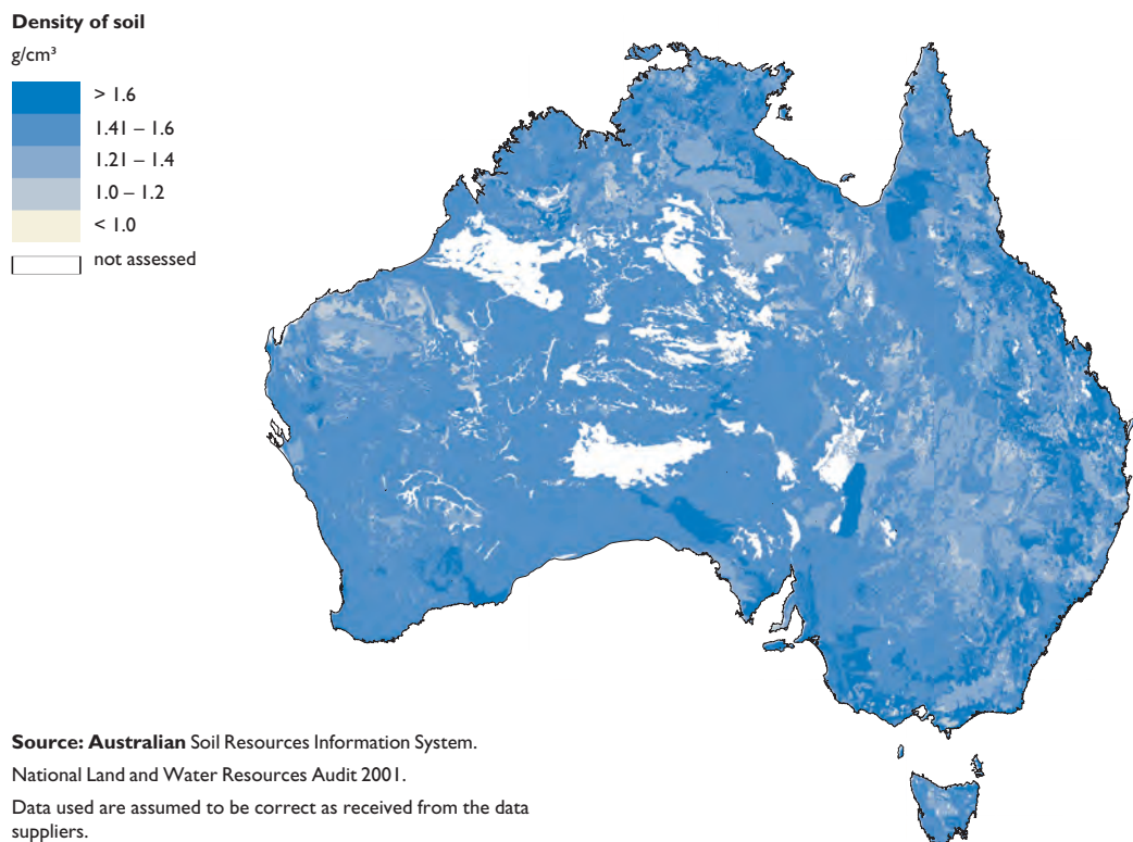
Figure A17 Distribution of bulk density ( \text{g/cm}^3 ) of the subsoil.
