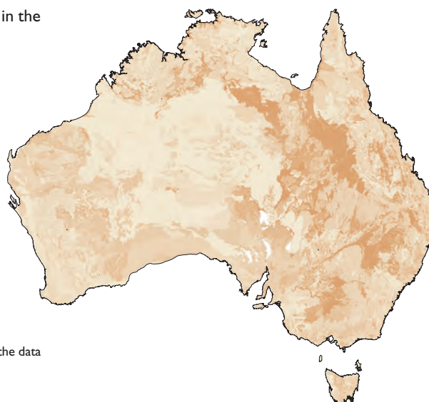
Figure A8 Distribution of percentage clay in the topsoil within the river basins containing intensive agriculture (point model).
