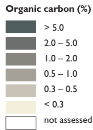
Figure A14 Distribution of organic carbon (%) in the topsoil within the river basins containing intensive agriculture.
