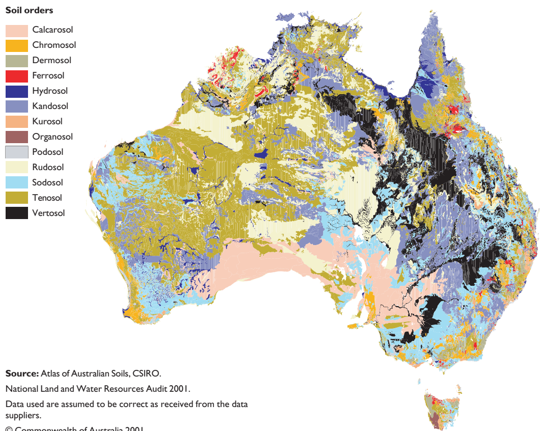
Figure A24 Distribution of soil orders in Australia.
