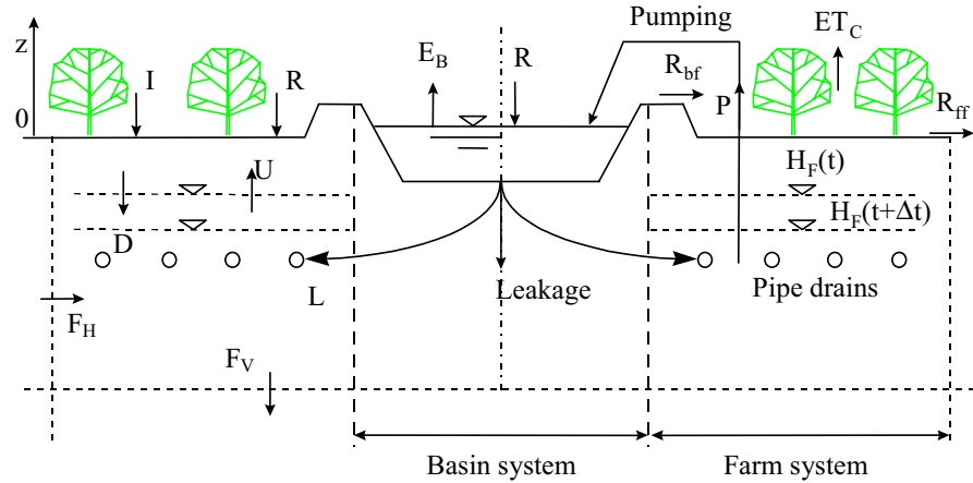
FIGURE 25. SCHEMATIC OF BASINMAN MODEL
