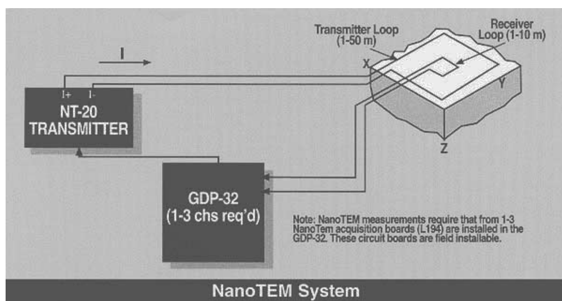
Figure 4.7 A schematic of the NanoTEM system in operation.
