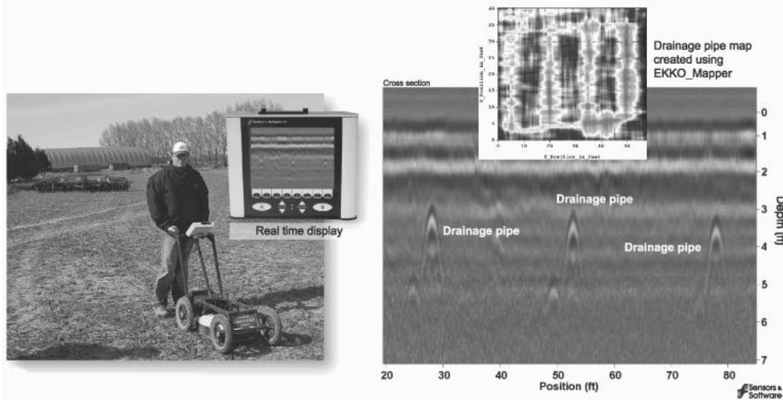
Figure 9.4 Sensors and Software Noggin ground penetrating radar system being used to locate agricultural tile drains.
