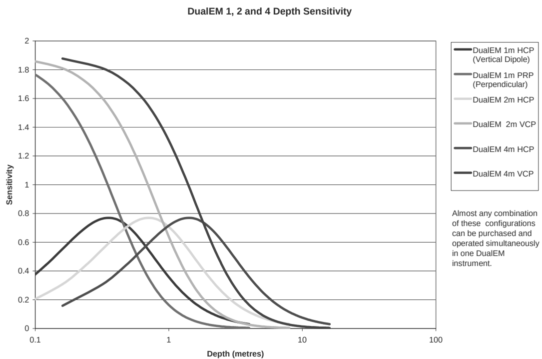
Figure 3.8 Depth sensitivities of the DUALEM instruments' configurations
