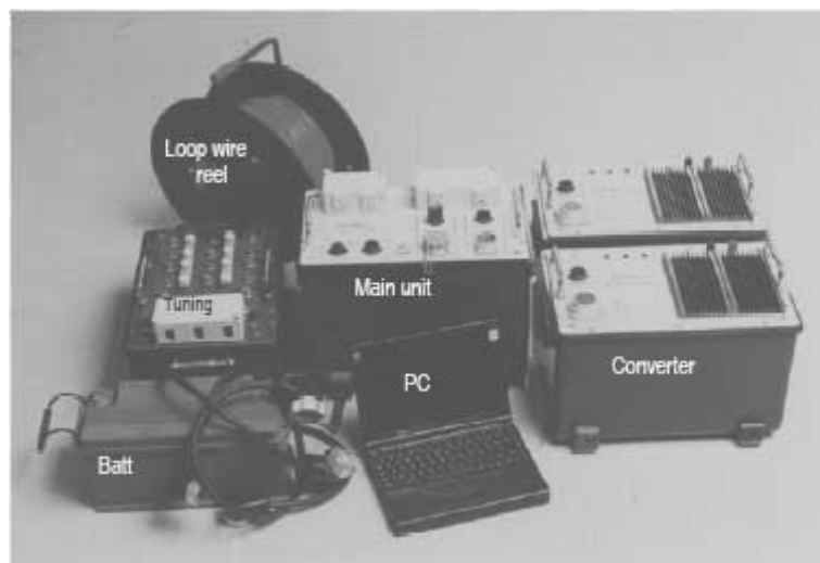
Figure 9.17 Iris Instruments Numis nuclear magnetic resonance sounding system
