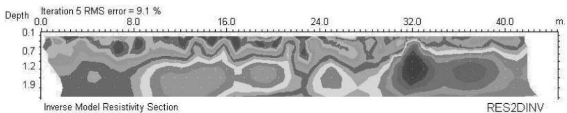
Figure 7.14 A sample of processed Corim data showing detailed variation in EC of a soil profile.
