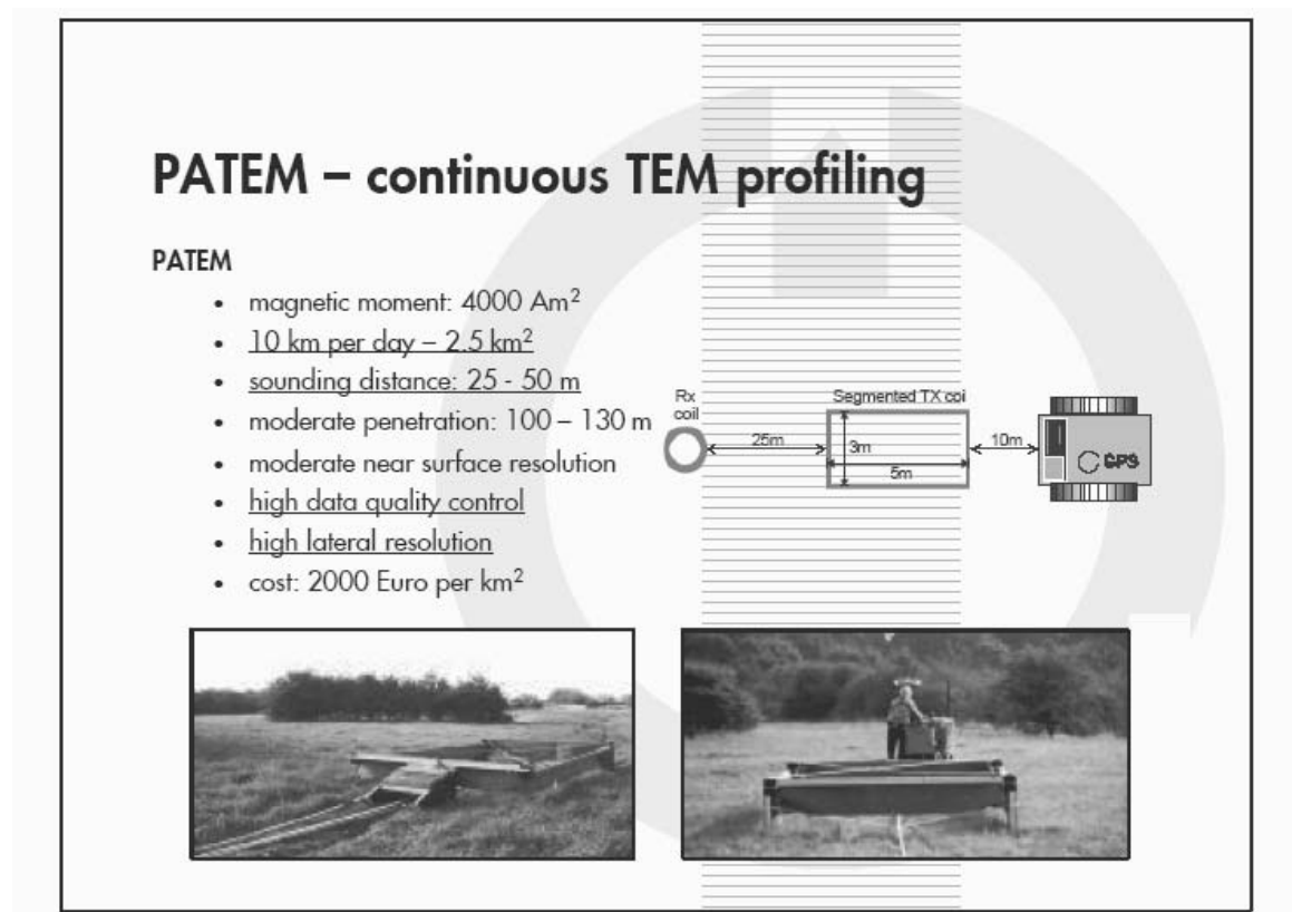
Figure 4.3 PATEM continuous profiling system
