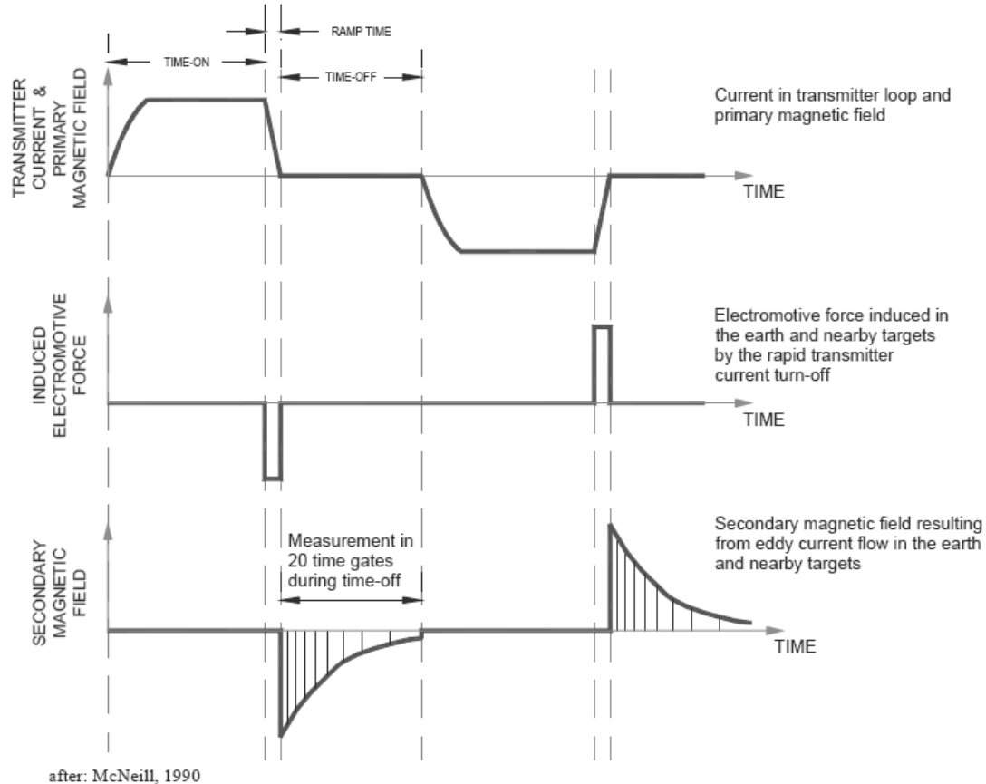
Figure 4.2 Waveforms in time domain electromagnetic systems. Note that EMF and secondary magnetic field produced by on time rise are not shown. (From http://www.nga.com/Flyers_PDF/NGA_TDEM_TEQ.pdf )
