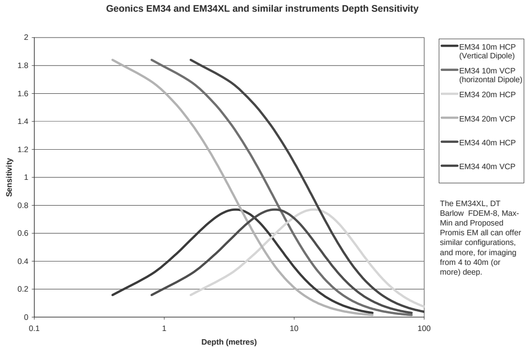
Figure 3.7 Depth Sensivities for the Geonics EM34 and EM34XL and similar instruments
