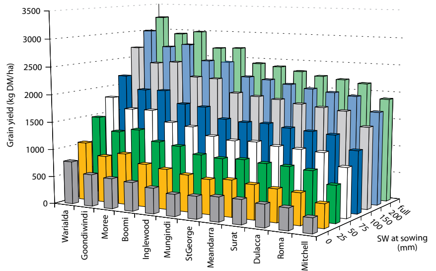
Simulated grain yields of wheat sown at eight levels of soil water on a grey vertosol at 12 locations throughout northern NSW and southern Queensland wheat-growing region.
