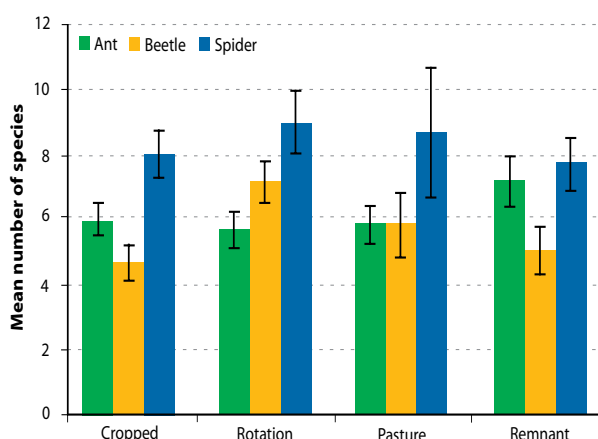
Avon invertebrate species diversity, Autumn 2006.
