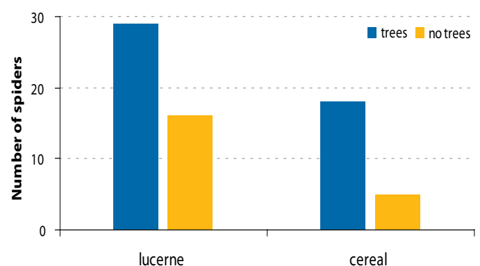
Crops with tree belts appear to have more spiders than those without trees. Source: A Cutler, P Horne, A Yen, M Elgar (2007) 'Spider populations in broadacre crops and pasture'
