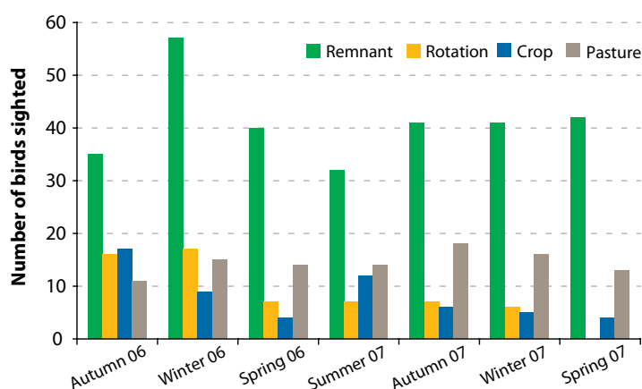
Avon bird species diversity.
