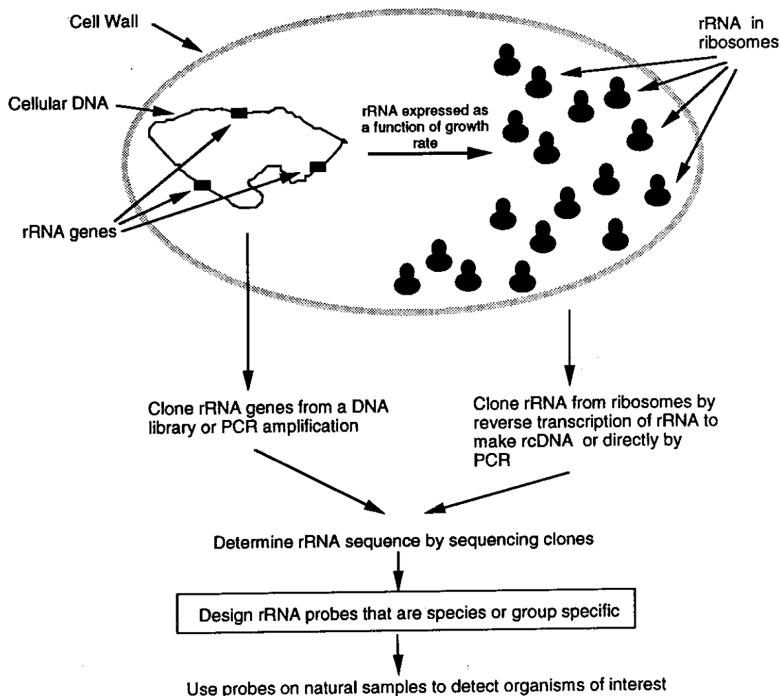
Figure 14: Ribosomal RNA expression and overview of strategy of rRNA probe design (modified from Ward et al. , 1992)
