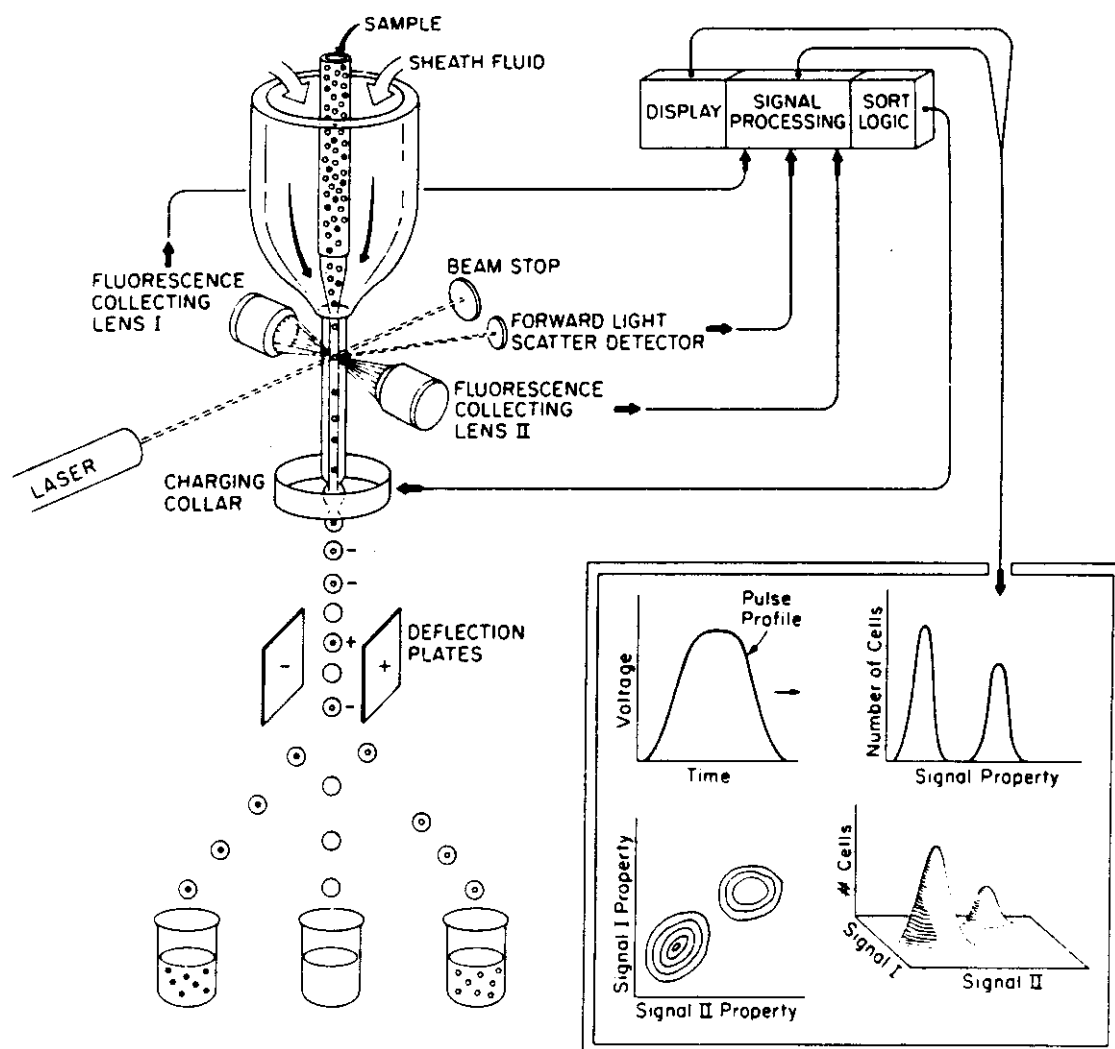
Figure 12: Flow cytometer/cell sorter (modified from Kemp et al. , 1993)
